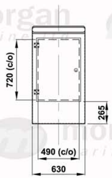
EXTERNAL VIEW WALL 1
