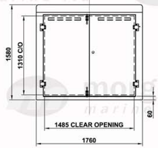
EXTERNAL VIEW WALL 1
