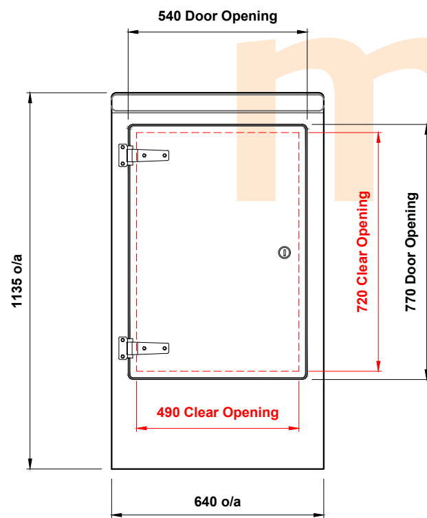
Elevation (A) (front) & Elevation (B) (rear)
