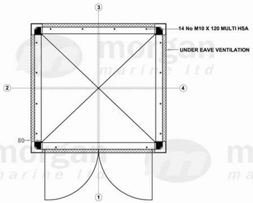
PLAN
