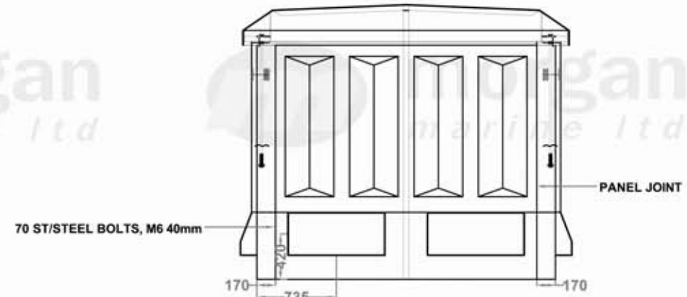
EXTERNAL ELEVATION WALL 03
