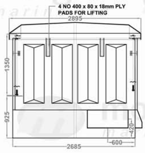
EXTERNAL ELEVATION WALL 04
